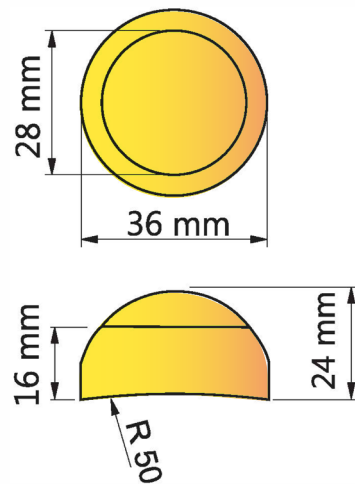
Safety caps for M10 and M12 screws
